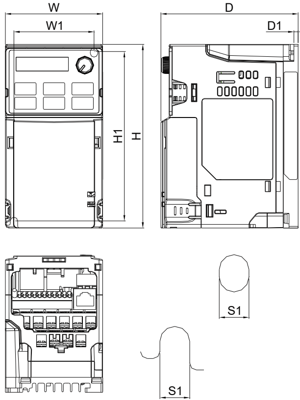
Mounting hole
